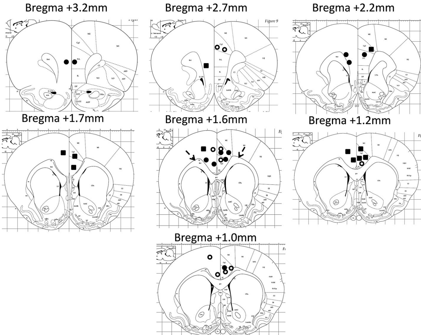
Figure 1 Schematic depicting of the sites of the bilateral injector placement in the rat medial prefrontal cortex (mPFC). Rats received microinjections of either vehicle (open circles) or GW6471 (closed circles) or GW7647 (closed squares) bilaterally into the mPFC. Bilateral off-target injection sites are indicated by black arrows. Images were taken from the rat brain atlas of Paxinos and Watson (2006).
